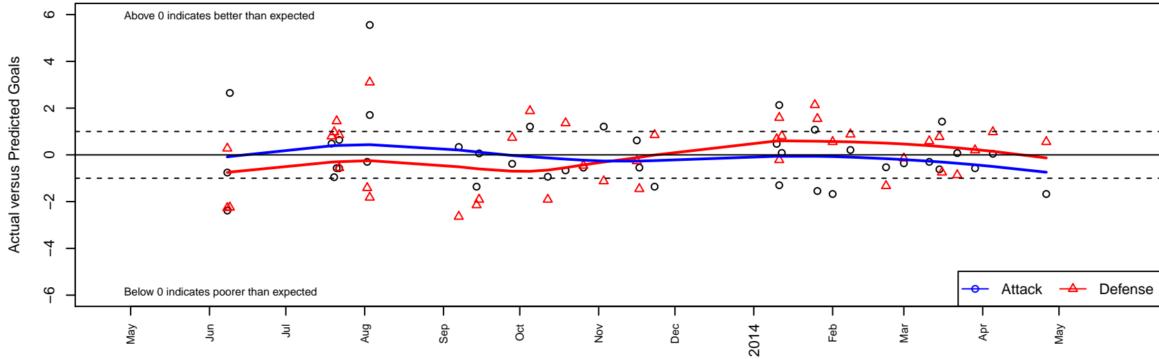
Crossfire Premier C G02 Dots are actual minus expected GF (blue circles) and GA (red triangles). Blue line is smoothed change in attack strength. Red is smoothed change in defense strength.
